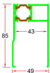
Bottom profile in 2 pieces
