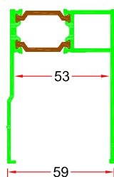
Bottom profile in 2 pieces
