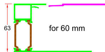
Side profile in 2 pieces
