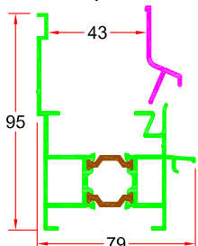
Bottom profile in 2 pieces
